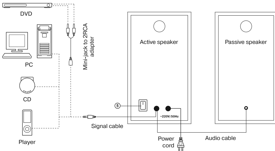
Fig. 2. Connection diagram
